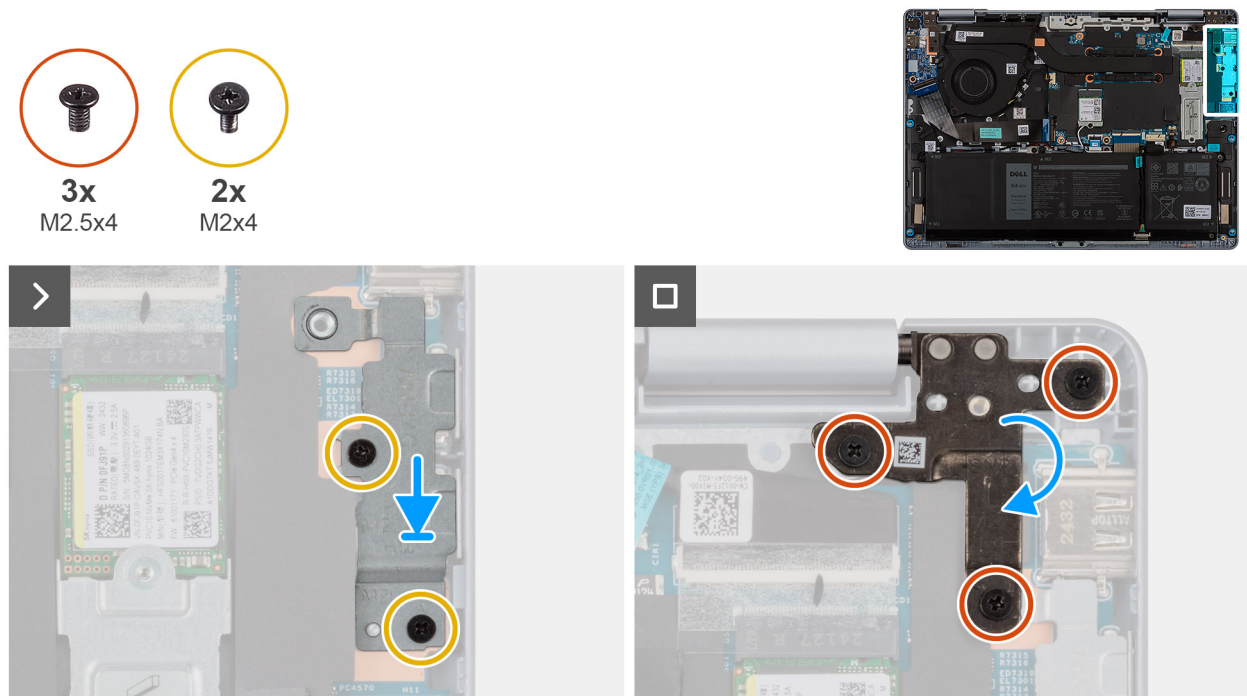
Figure 37. Installing the USB Type-C bracket
