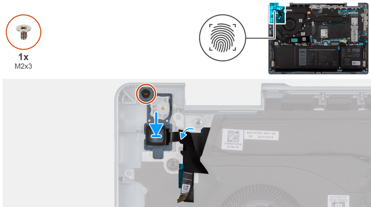
Figure 35. Installing the power button with fingerprint reader
